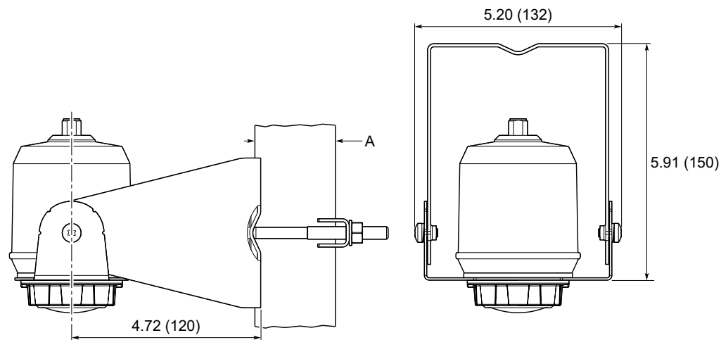
Figure 12: Standard Version
