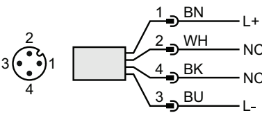
Figure 4: Connection
