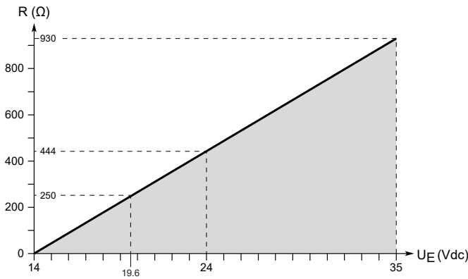
Figure 3: Load Limits
