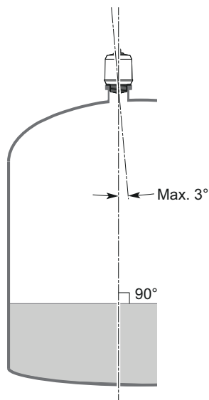
Figure 7: Inclination
