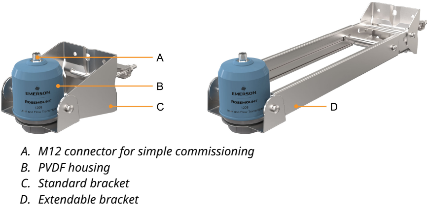
Figure 1: Bracket Mounting
