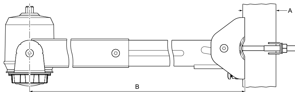
Figure 13: Extendable Version
