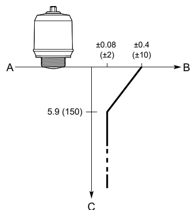
Figure 2: Accuracy Over Measuring Range
